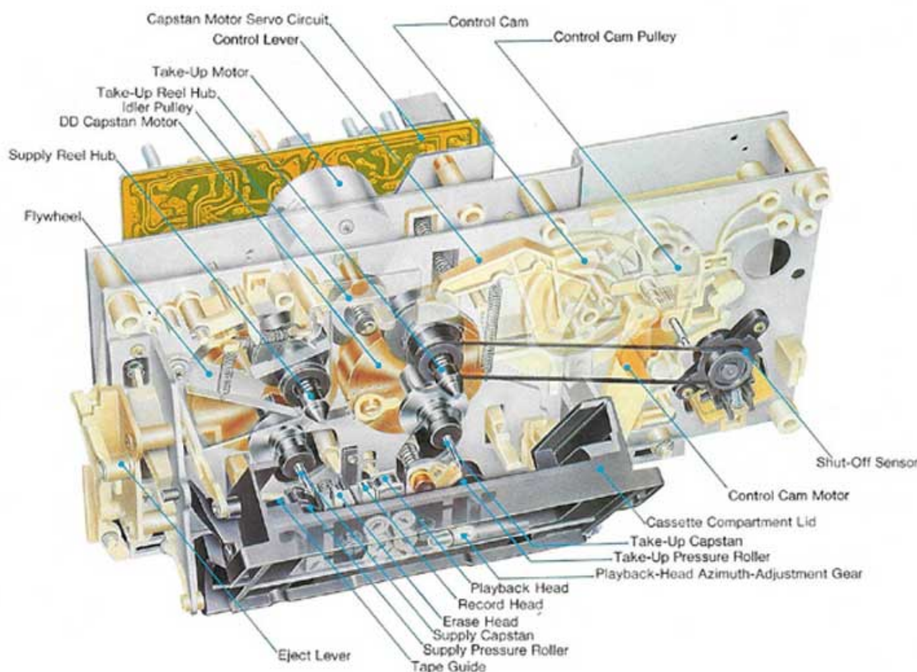
Transport Mechanism Construction Diagram
