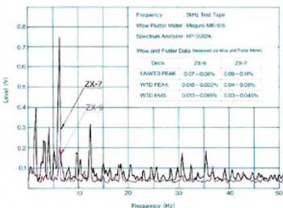
Flutter Spectral Analysis (UNWTD Peak)
