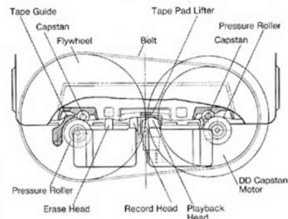
Direct-Drive Dual-Capstan Configuration
